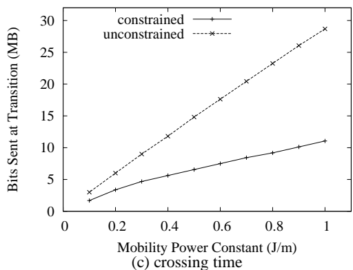
Figure 17: Performance improvement of mobility control in networks with multiple flows.
