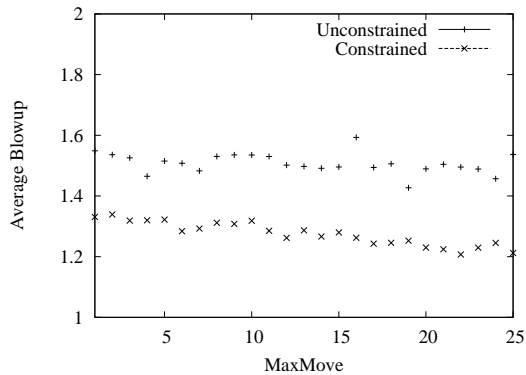
Figure 8: Blowup of network path.
